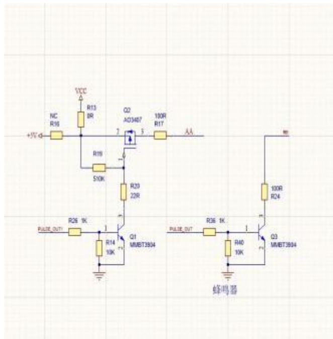
Interface diagram (shown from the back of the module)
